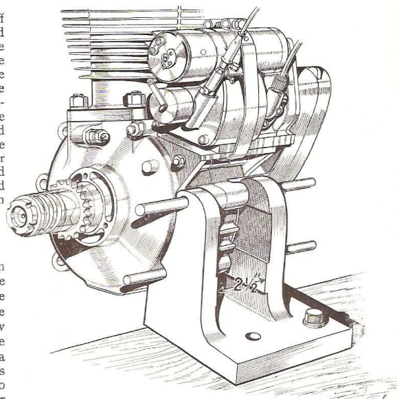
Fig. M15. Angle bracket for mounting engine.
